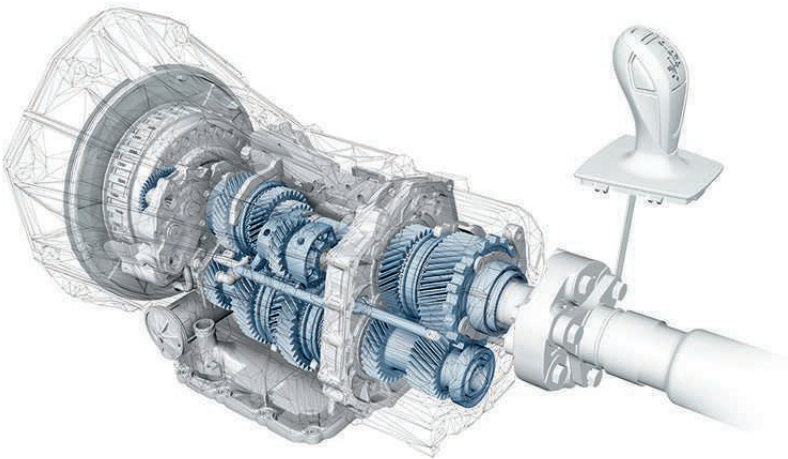
In the seven-speed sport automatic transmission with double clutch, even and uneven gears are distributed across two power trains. So while one gear is being disengaged, the next is already in position – meaning the fastest of shifts with a maximum of precision.
