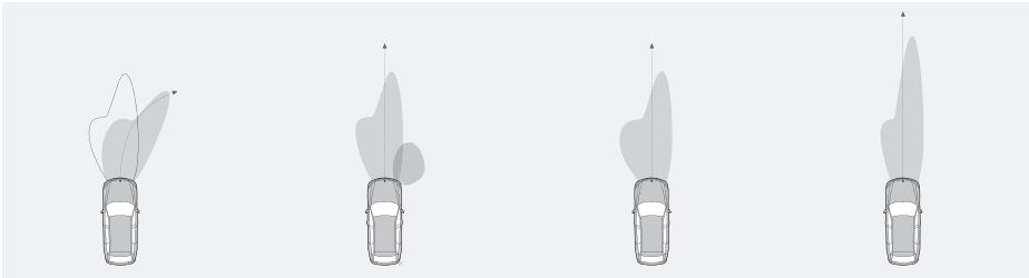
Adaptive Headlights: the headlights are directed into the bend ahead. Cornering lights: for improved sideways illumination when turning at low speeds. Country/urban mode: for improved illumination of the far side of the road. Motorway mode: extends the range of the headlights.
